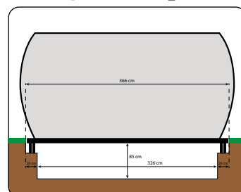
Scheme of immersion of the trampoline in the ground
